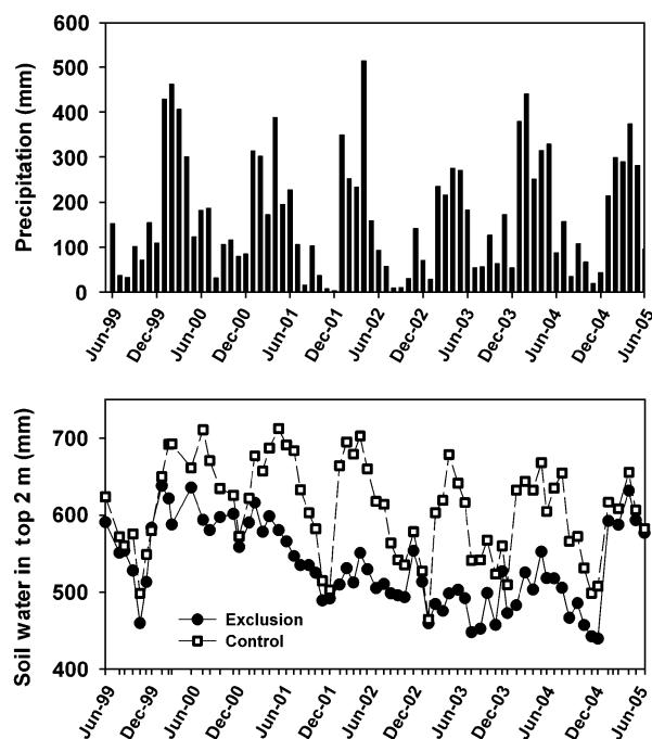
Fig. 1 Monthly precipitation (a) and volumetric water content of the top 2 m of soil (b). The throughfall exclusion treatment was applied during the rainy seasons of 2000–2004.
