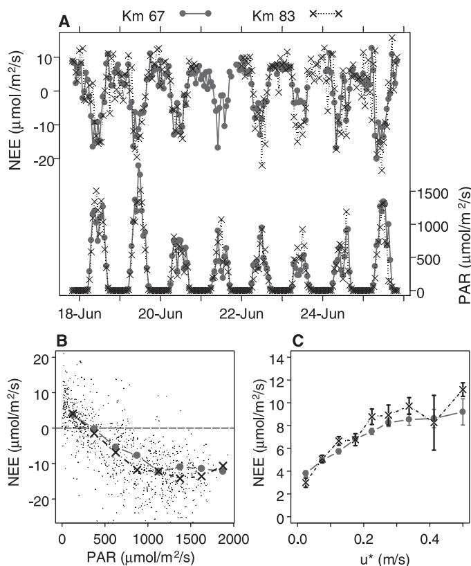
Fig. 1. Comparison between km 83 and km 67 tower sites. (A) Coherent time series for NEE and sunlight [photosynthetically active radiation (PAR)]. (B) Similar curves for daytime NEE versus PAR. (C) Nighttime NEE versus friction velocity ( u^* ). Declining NEE at u^* < 0.2 is evidence that tower measurements underestimate NEE during calm conditions at night.
