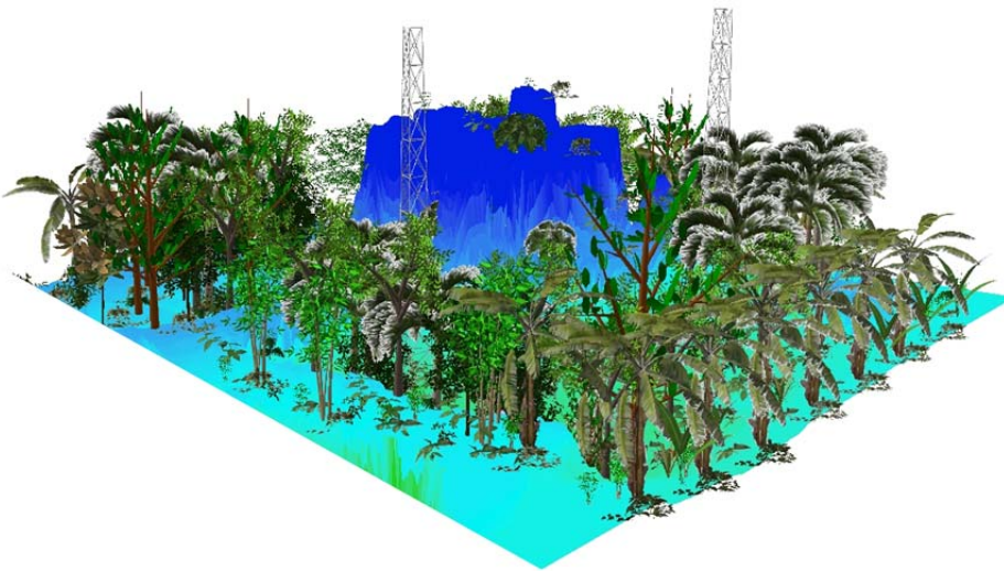
Figure 2: Snapshot from the three-dimensional version of the B2 tropical rainforest map in Arc-GIS. Visible in the center is the “mountain”. Tree and profile tower models imported from Google Sketchup.
