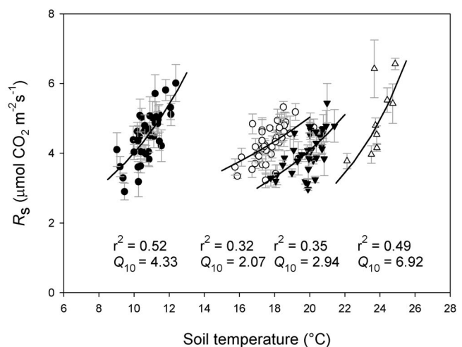
Figure 4. Temperature dependence of total soil respiration (with standard errors) at 3030 m asl (solid circles), 1500 m asl (open circles), 1000 m asl (solid inverted triangles), and 200 m asl (open triangles) for the year 2008 together with fitted Lloyd and Taylor [1994] functions and Q_{10} values as calculated for site specific mean annual temperatures ( T_s ) \pm 5^\circ\text{C} .
